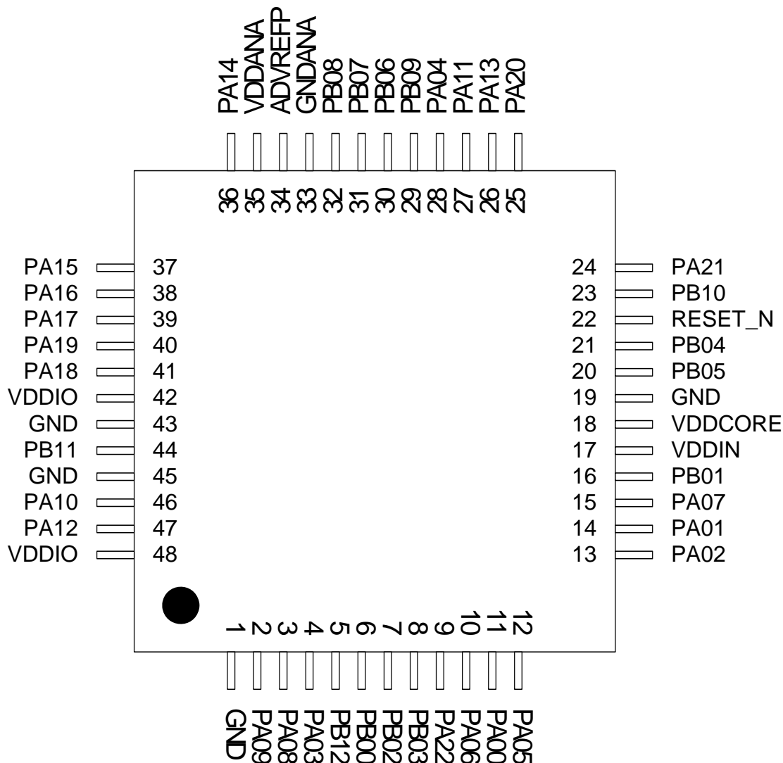
Figure 3-1. TQFP48/QFN48 Pinout
