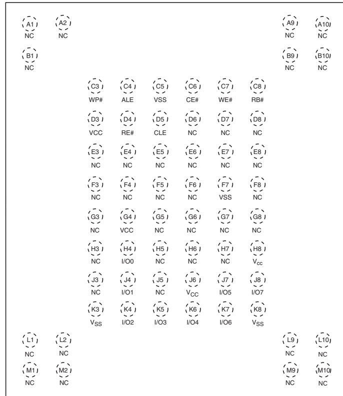
Figure 1.2 63-BGA Contact, x8 Device, Single CE (Top View)
