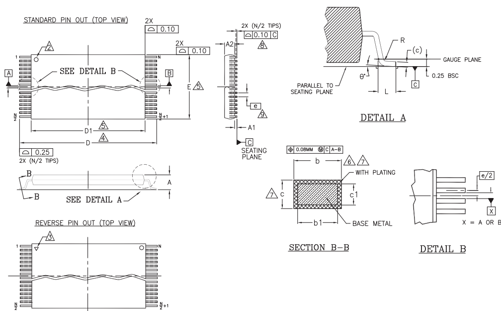
Figure 8.1 TS2 48 — 48-lead Plastic Thin Small Outline, 12 x 20 mm, Package Outline
