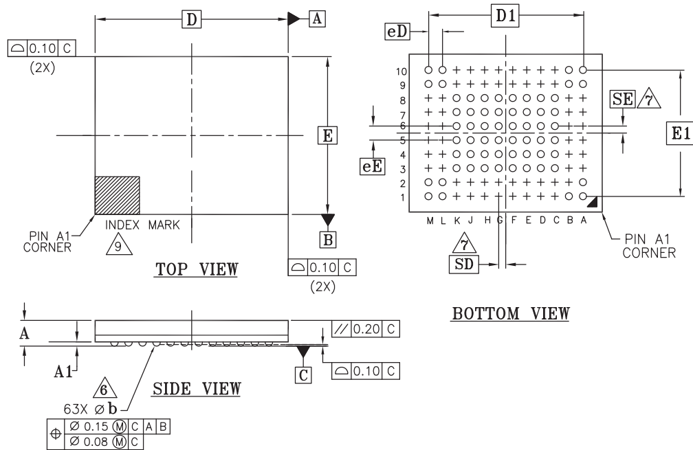
Figure 8.2 VLD063 — 63-Pin BGA, 11 mm x 9 mm Package
