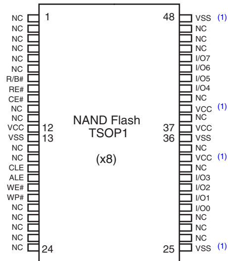
Figure 1.1 48-Pin TSOP1 Contact x8 Device (1 CE 8 Gb)
