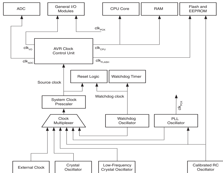
Figure 6-1. Clock Distribution
