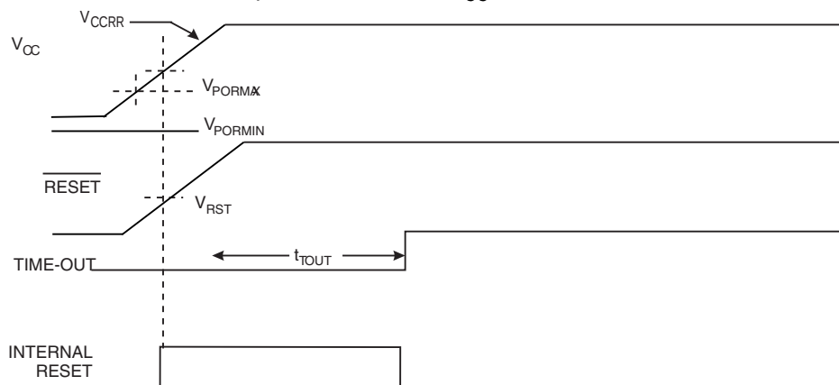
Figure 8-2. MCU Start-up, \overline{\text{RESET}} Tied to V_{CC}
