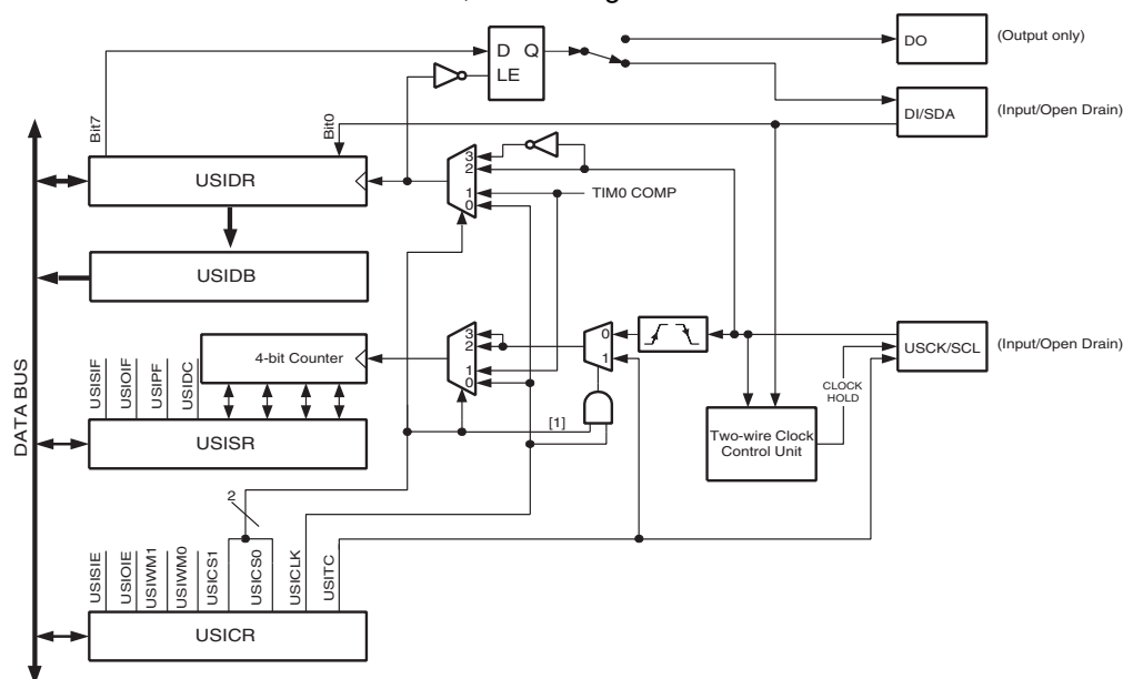
Figure 16-1. Universal Serial Interface, Block Diagram
