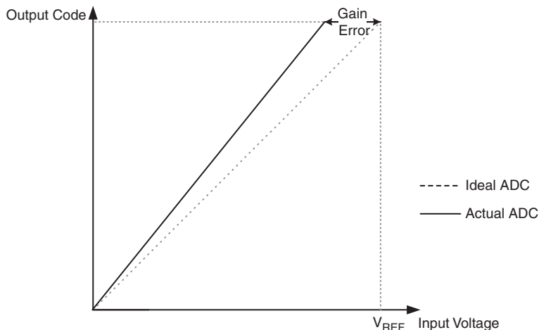
Figure 18-10. Gain Error
