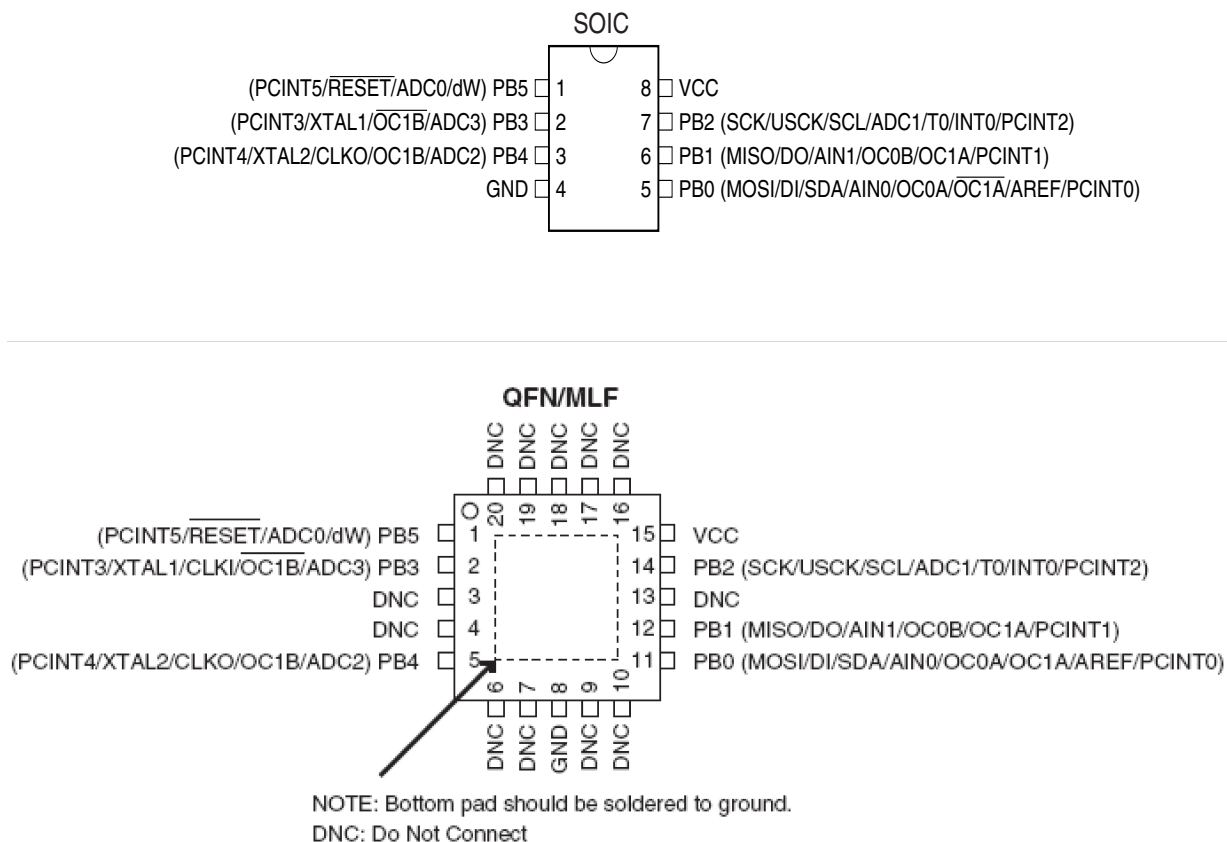
Figure 1-1. Pinout ATtiny25/45/85
