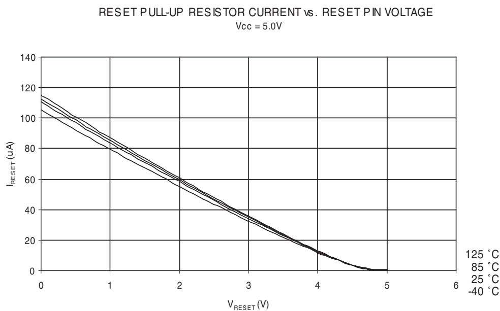
Figure 23-18. Reset Pull-Up Resistor Current vs. Reset Pin Voltage ( V_{CC} = 5.0V )
