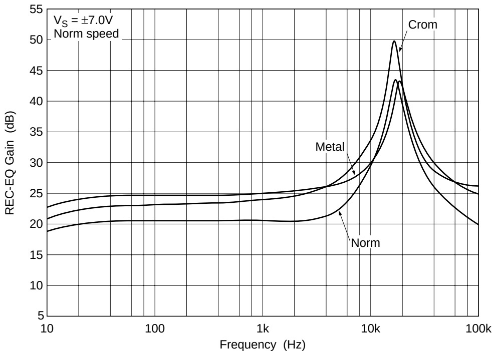
Equalizer Amp. Gain vs. Frequency (1)
