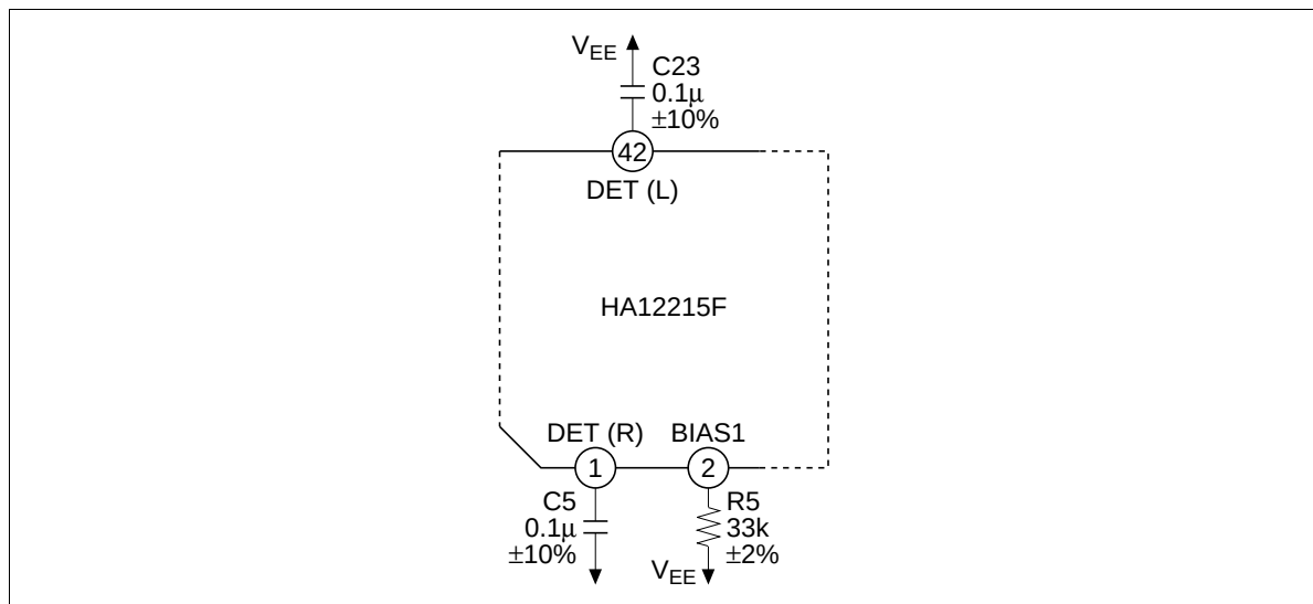
Figure 7 Tolerance of External Components
