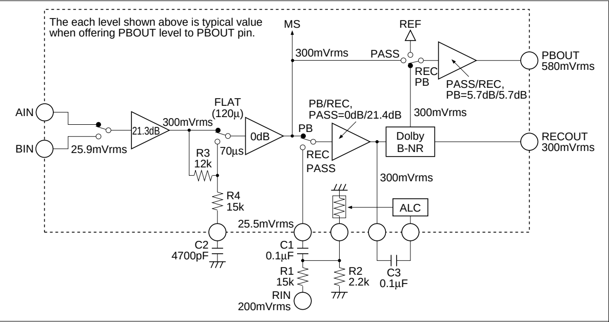
Figure 2 Input Block Diagram
