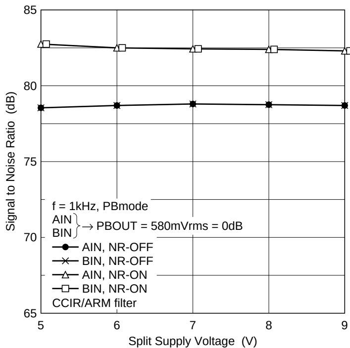
Signal to Noise Ratio vs. Split Supply Voltage (2)
