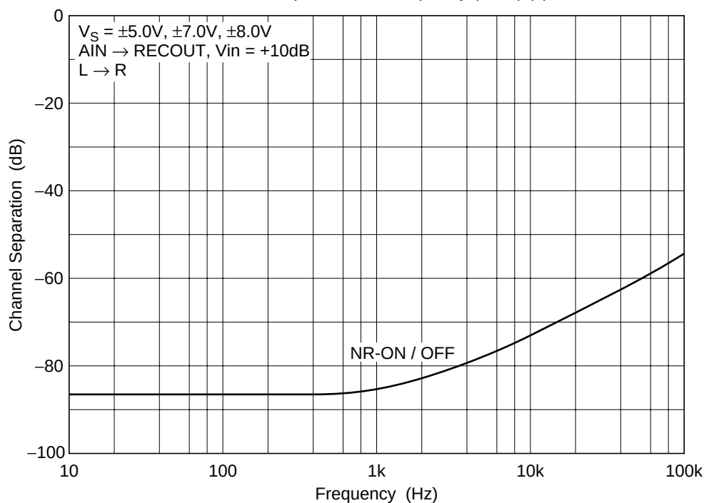
Channel Separation vs. Frequency (L→R) (6)
