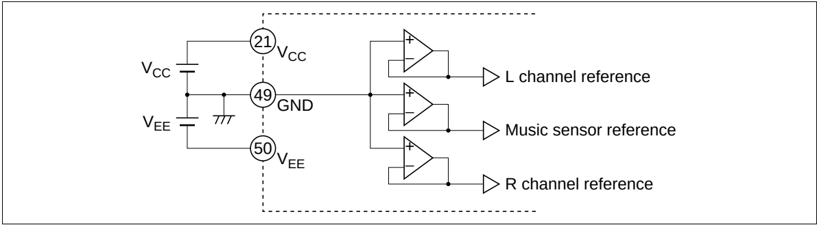
Figure 1 Reference Voltage
