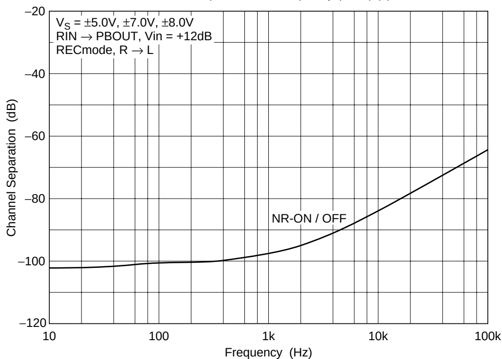
Channel Separation vs. Frequency (R→L) (2)
