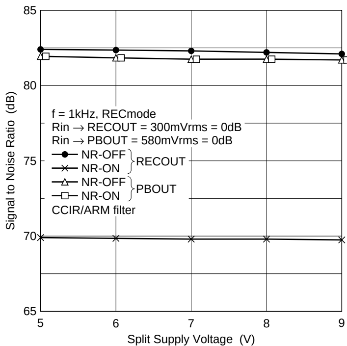
Signal to Noise Ratio vs. Split Supply Voltage (1)
