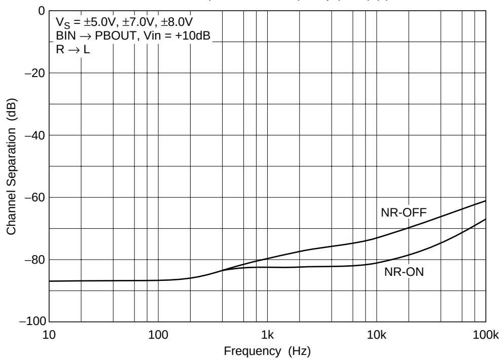
Channel Separation vs. Frequency (R→L) (3)
