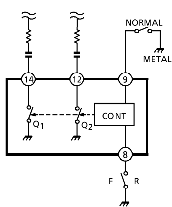
Fig.1 Equalizer switchover function
