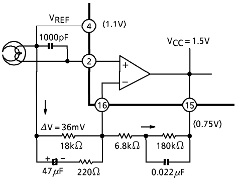
Fig.4 NFB terminal
