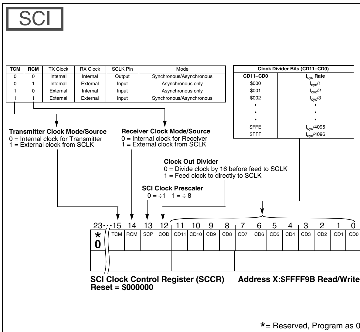
Figure B-18. SCI Clock Control Registers (SCCR)
