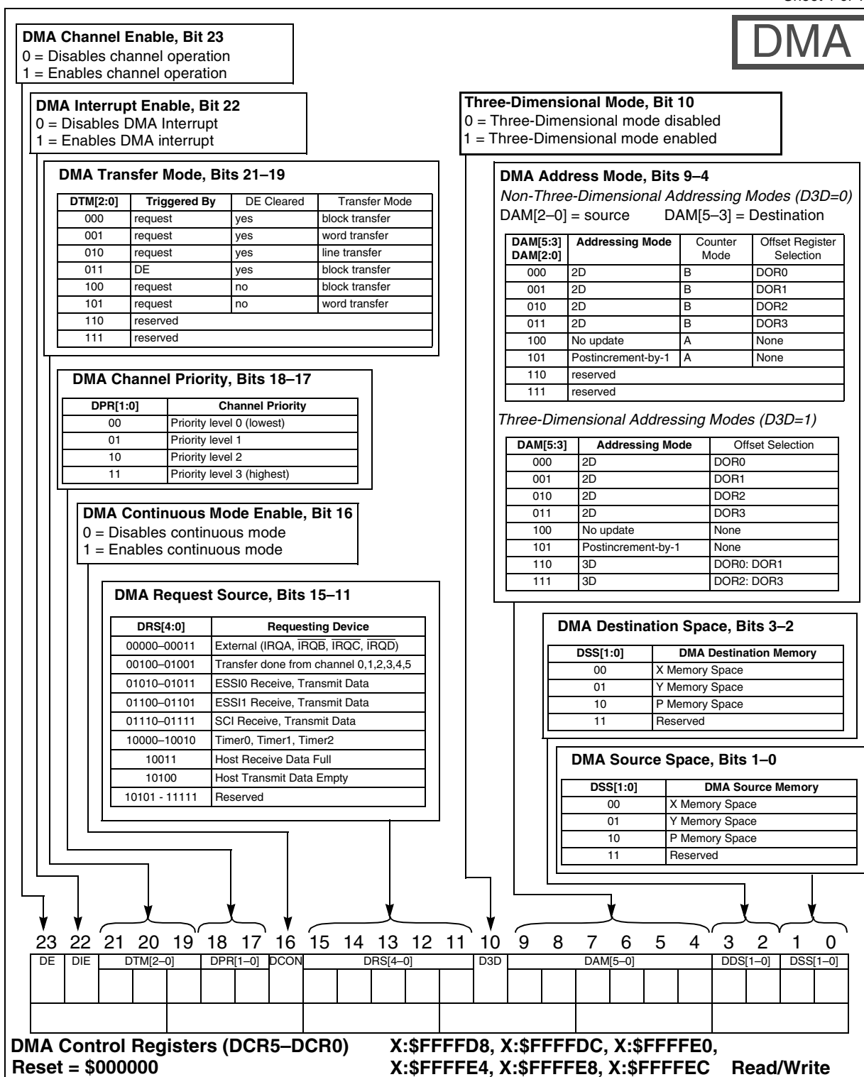
Figure B-8. DMA Control Registers 5–0 (DCR[5–0])
