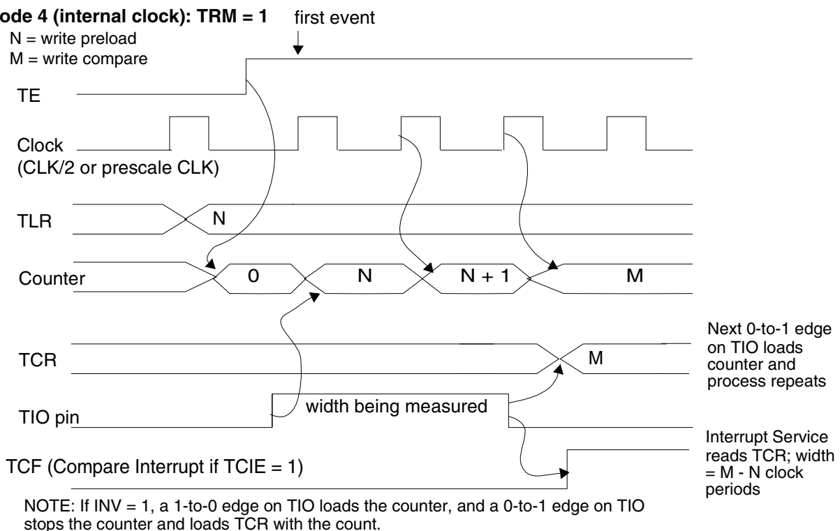
Figure 9-11. Pulse Width Measurement Mode, TRM = 1
