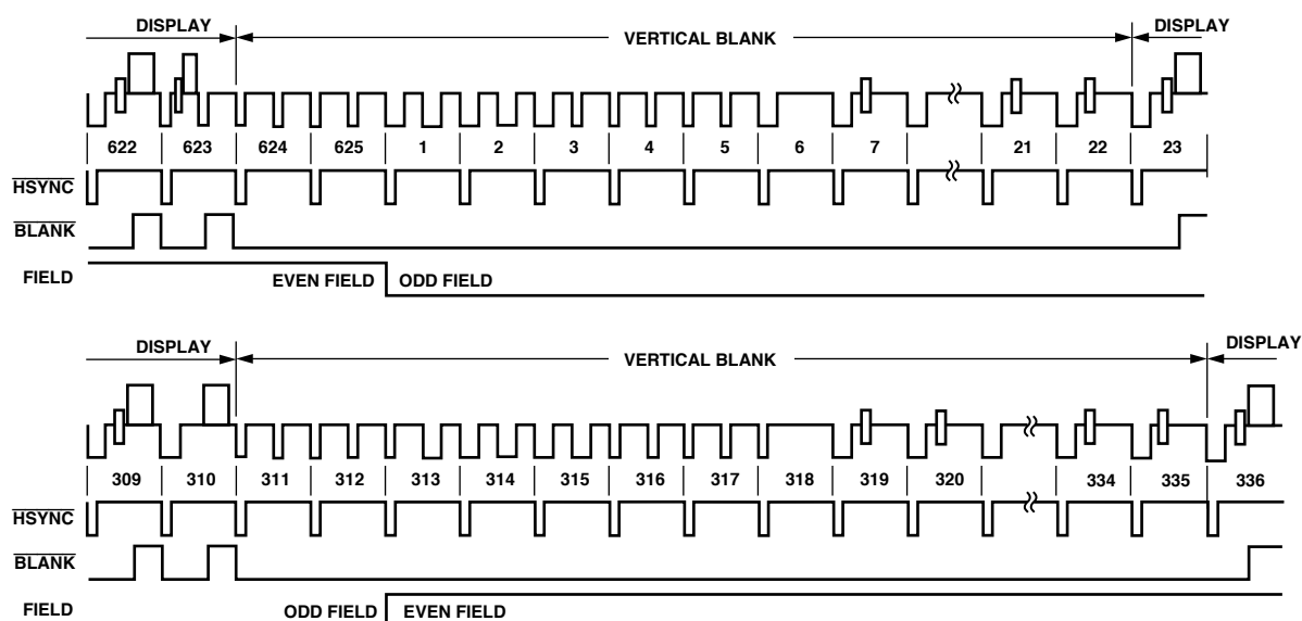
Figure 38. Timing Mode 1, PAL
