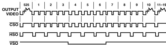
Figure 29. \overline{\text{CSO}} , \overline{\text{HSO}} , \overline{\text{VSO}} Timing Diagram
