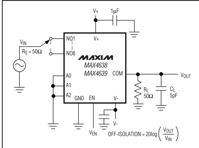
Figure 6. Off-Isolation/On-Channel Bandwidth
