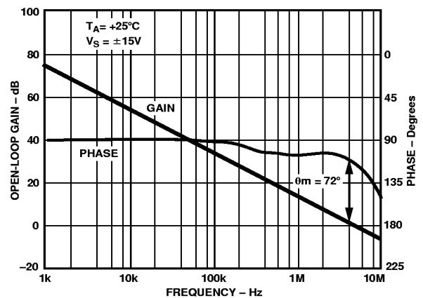
Figure 24. Open-Loop Gain, Phase vs. Frequency @ \pm 15 V
