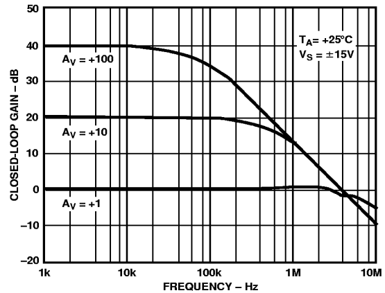
Figure 25. Closed-Loop Gain vs. Frequency @ \pm 15 V
