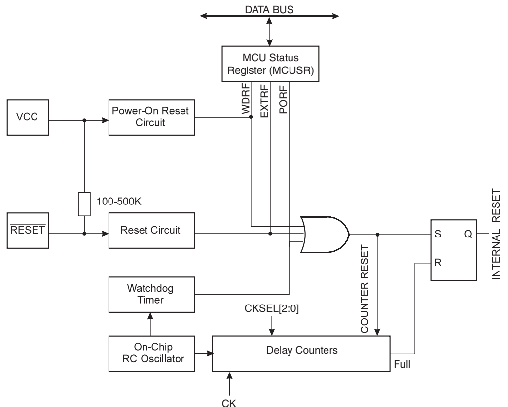
Figure 24. Reset Logic
