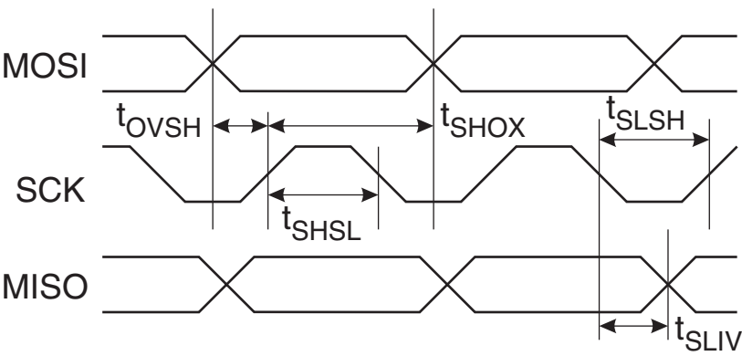
Figure 81. Serial Programming Timing
