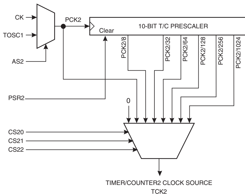
Figure 30. Timer/Counter2 Prescaler
