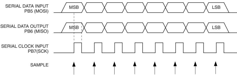
Figure 80. Serial Programming Waveforms
