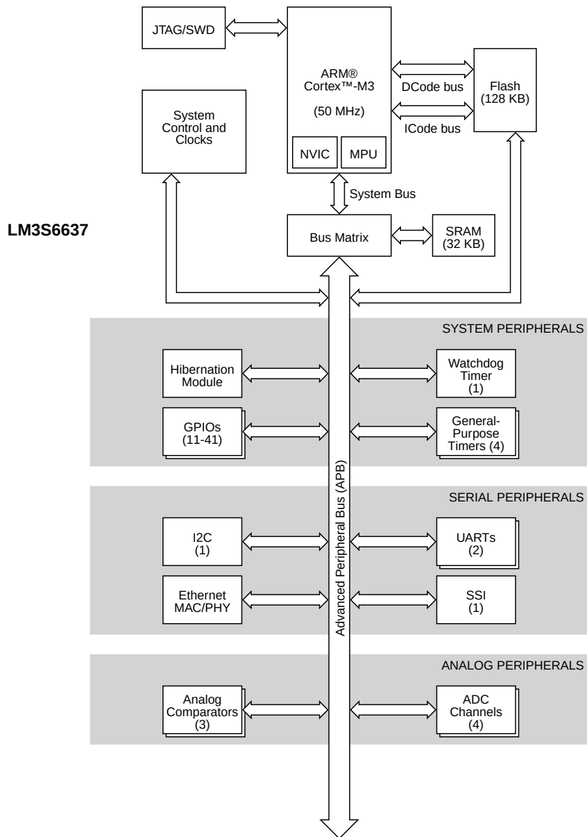
Figure 1-1. Stellaris® LM3S6637 Microcontroller High-Level Block Diagram
