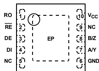
ISL3159E (10 LD DFN) TOP VIEW
