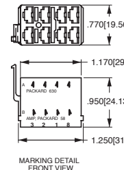
VCH CONNECTOR HOUSING
