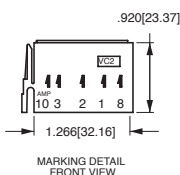
VC2 CONNECTOR HOUSING (For AMP terminals only)
