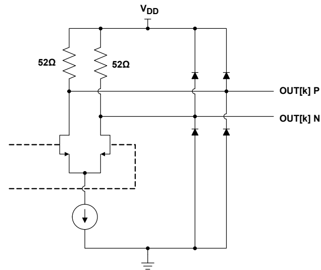
FIGURE 26. CML OUTPUT EQUIVALENT CIRCUIT FOR THE QLx4600-SL30 NOTE: The load value of 52Ω is used to internally match S DD22 for a characteristic impedance of 50Ω.
