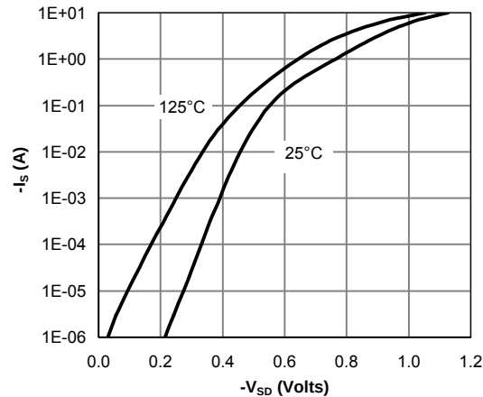
Figure 6: Body-Diode Characteristics
