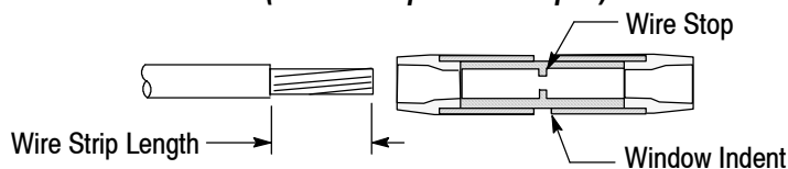
Typical Splice (Without Step-Down Adapter)
