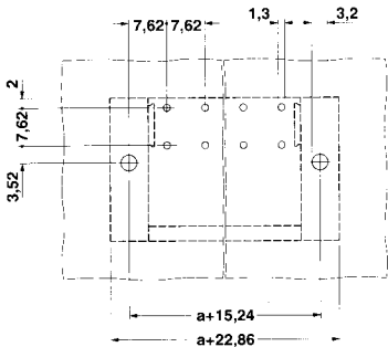
Drilling diagram PC 4/...-G (with BF-PC 4)
