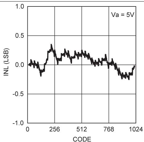
Figure 3. Define (INL)
