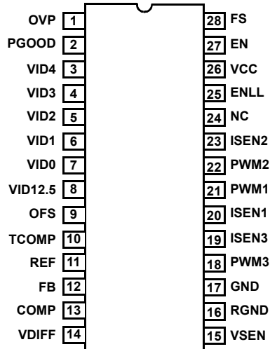
ISL6565ACB (SOIC), ISL6565ACV (TSSOP) TOP VIEW
