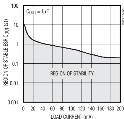
REGION OF STABLE ESR vs. LOAD CURRENT
