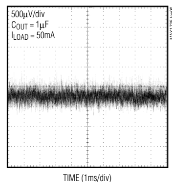
OUTPUT NOISE (10Hz TO 1MHz)
