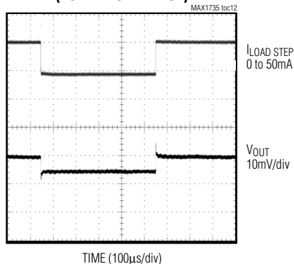
LOAD-TRANSIENT RESPONSE (NORMAL OPERATION)
