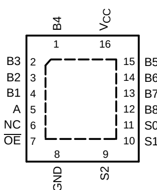
RGY PACKAGE (TOP VIEW)
