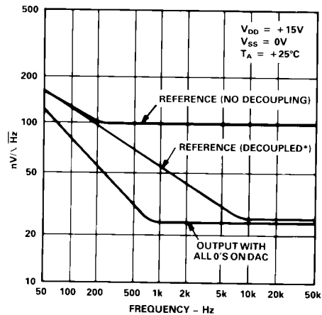
Noise Spectral Density vs. Frequency
