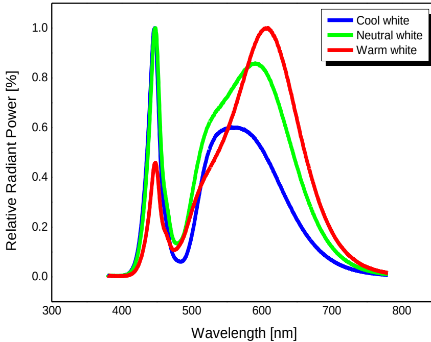
Fig 1. Color Spectrum, T_a = 25^{\circ}\text{C} , I_F = 700\text{mA} , RH30%
