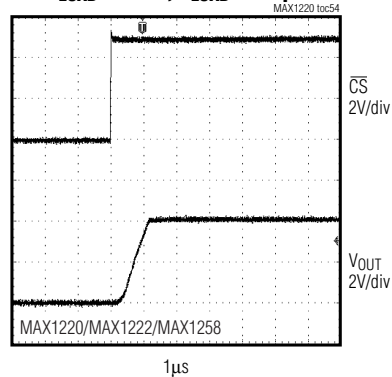
DYNAMIC RESPONSE RISE TIME RLOAD = 10kΩ, CLOAD = 100pF
