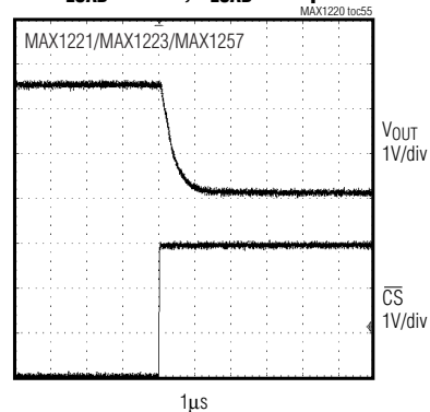
DYNAMIC RESPONSE FALL TIME RLOAD = 10kΩ, CLOAD = 100pF
