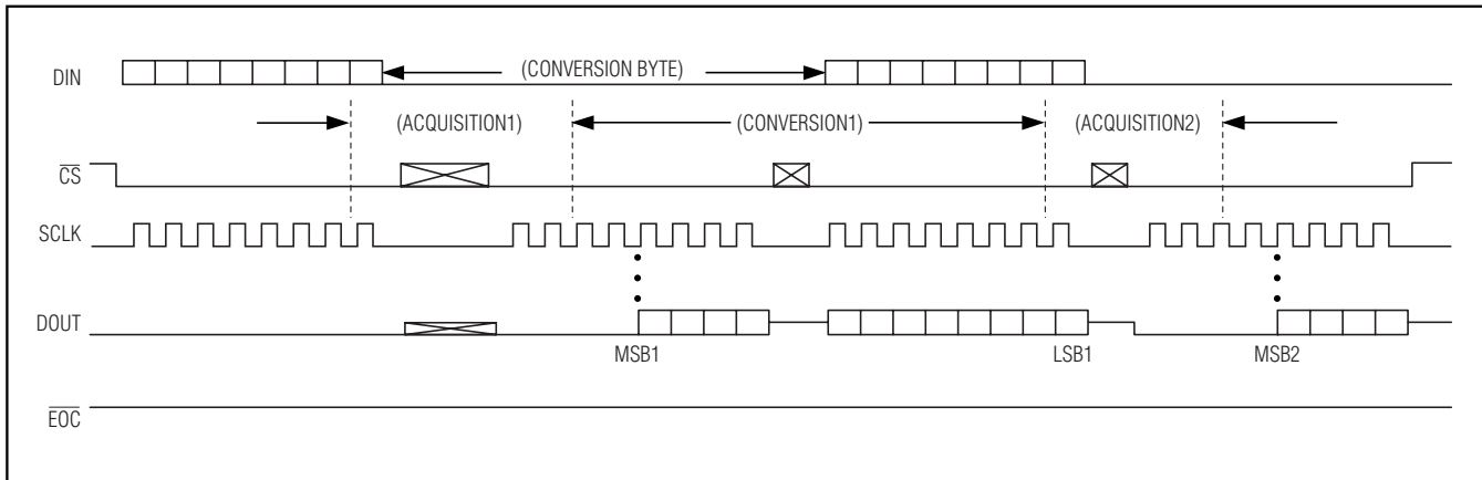
Figure 9. Clock Mode 11—Externally Timed Acquisition, Sampling, and Conversion without \overline{\text{CNVST}}
