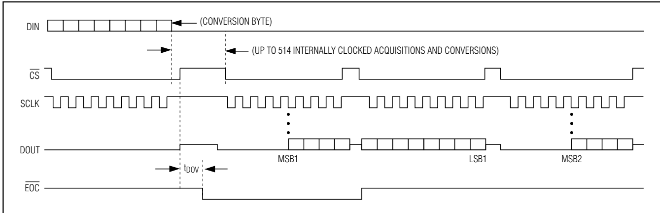
Figure 8. Clock Mode 10—The command byte to the conversion register begins the acquisition ( \overline{\text{CNVST}} is not required).
