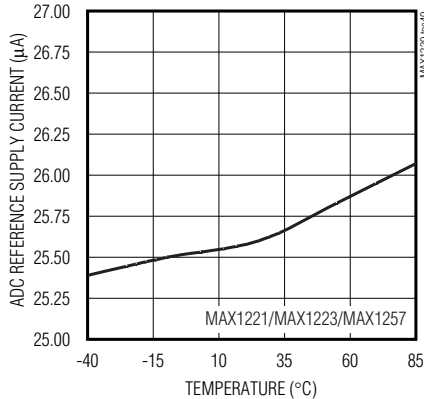
ADC REFERENCE SUPPLY CURRENT vs. TEMPERATURE
