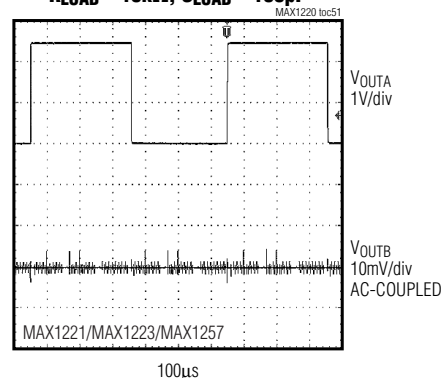
DAC-TO-DAC CROSSTALK RLOAD = 10kΩ, CLOAD = 100pF
