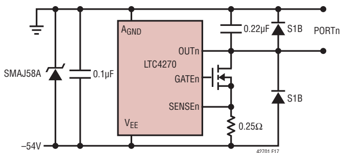
Figure 16. LTC4270 Discharge Protection
