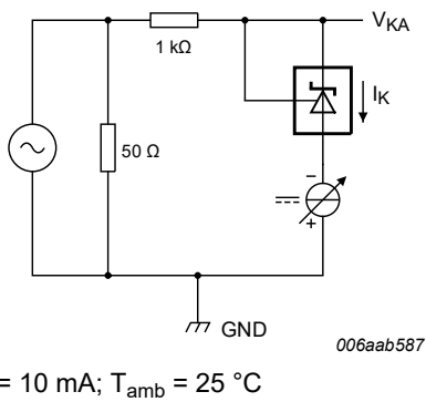
Fig. 16. Test circuit to Figure 15
