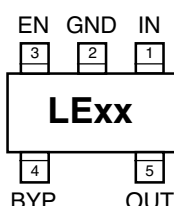
MIC5207-x.xBM5 SOT-23-5 MIC5207-x.xBD5 TSOT-23-5 (Fixed Voltages)
