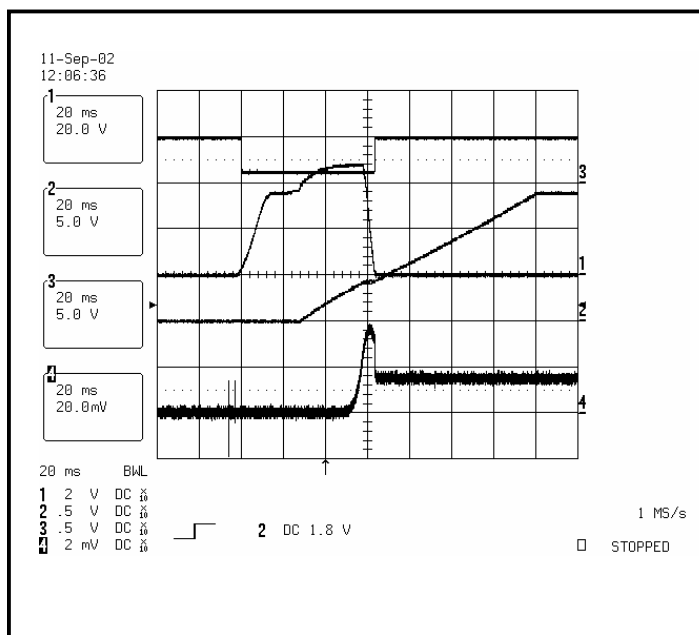
Figure 6. Start-up with 1A load.
