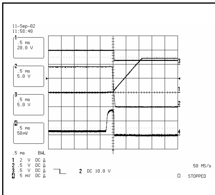
Figure 8. Over-current/Short circuit.
