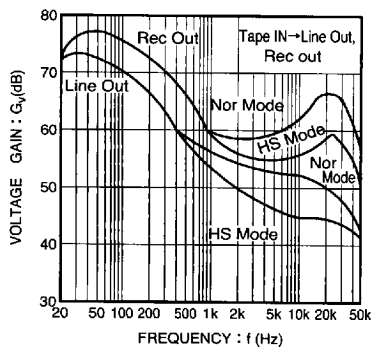
Fig. 14 Voltage gain vs. frequency
