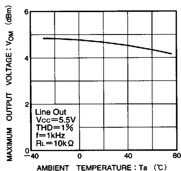
Fig. 5 Maximum output voltage vs. ambient temperature
