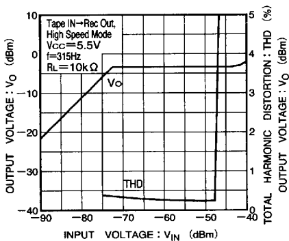
Fig. 9 Output voltage vs. input voltage
