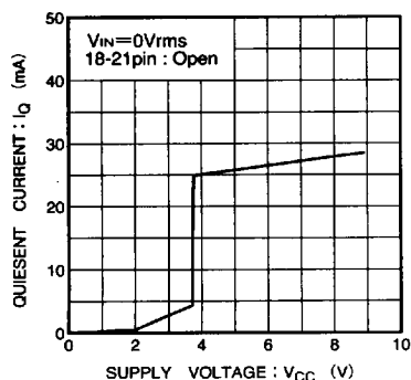
Fig. 2 Quiescent current vs. supply voltage
