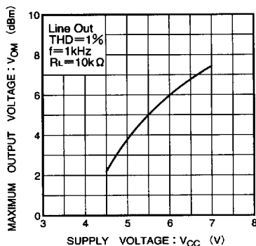
Fig. 3 Maximum output voltage vs. supply voltage
