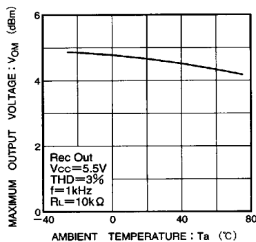
Fig. 6 Maximum output voltage vs. ambient temperature
