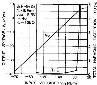
Fig. 11 Output voltage vs. input voltage
