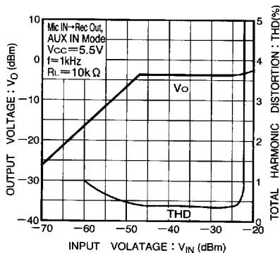
Fig. 12 Output voltage vs. input voltage
