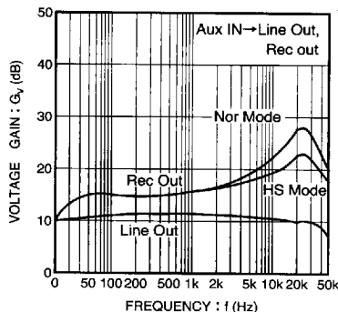
Fig. 15 Voltage gain vs. frequency
