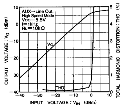
Fig. 8 Output voltage vs. input voltage
