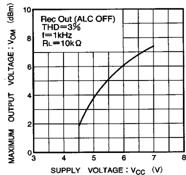
Fig. 4 Maximum output voltage vs. supply voltage
