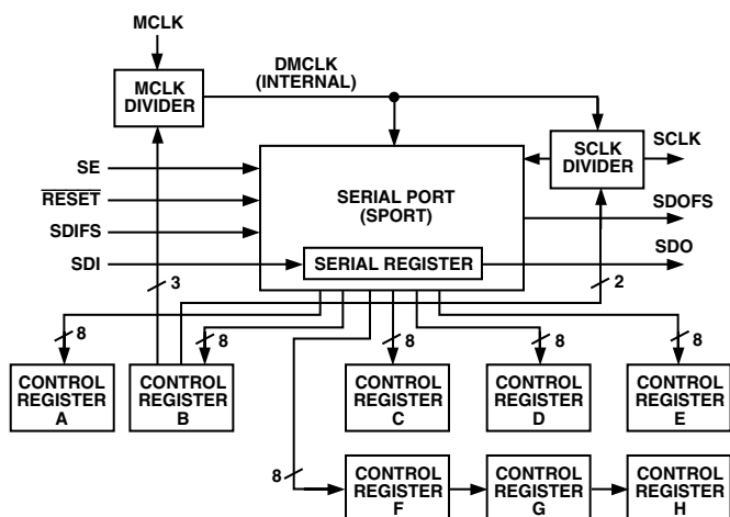
Figure 9. SPORT Block Diagram
