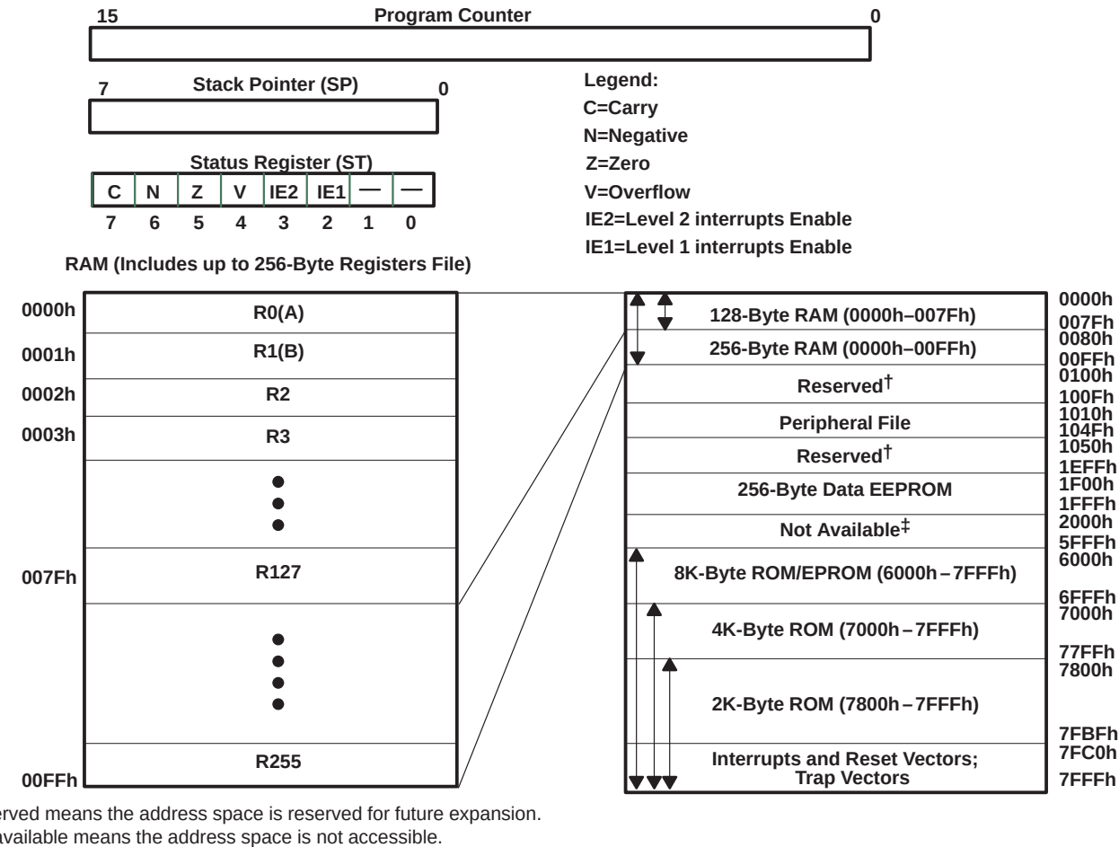
Figure 1. Programmer's Model
