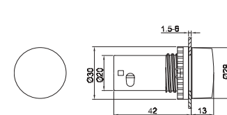
Pilot light
