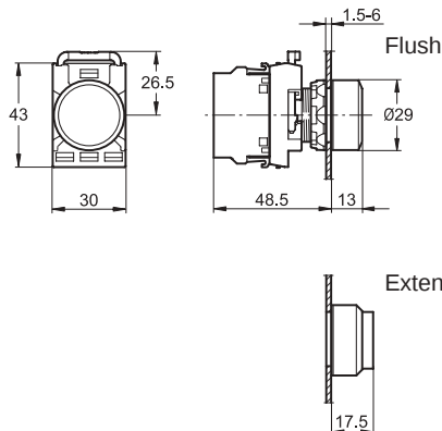
Pushbutton
