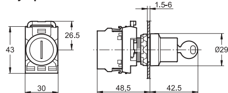
Key-operated selector switch
