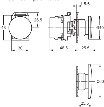
Mushroom pushbutton
