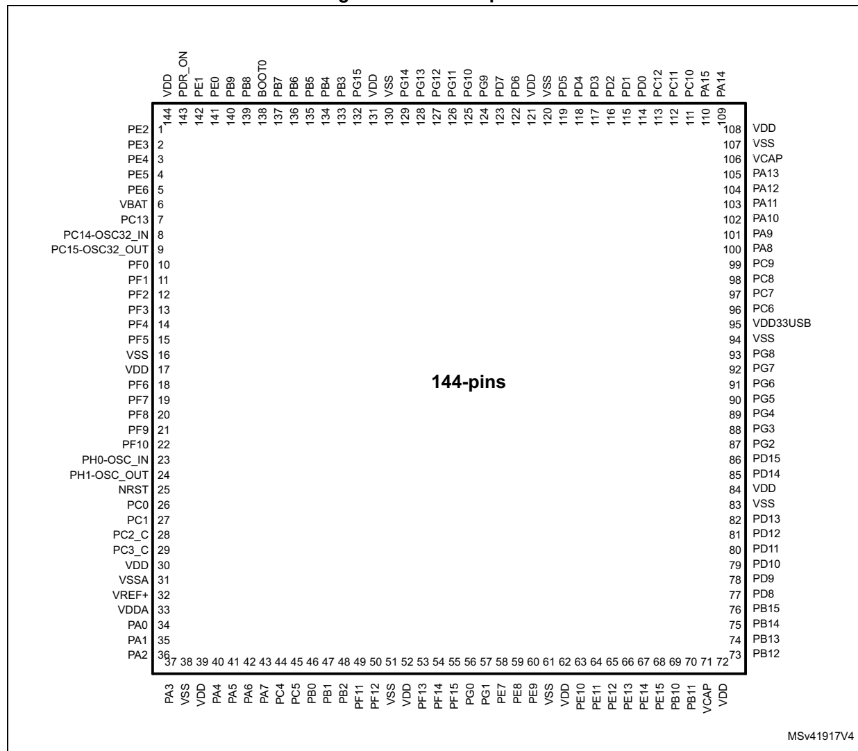
Figure 6. LQFP144 pinout
