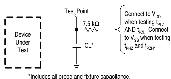
Figure 7. Test Circuit
