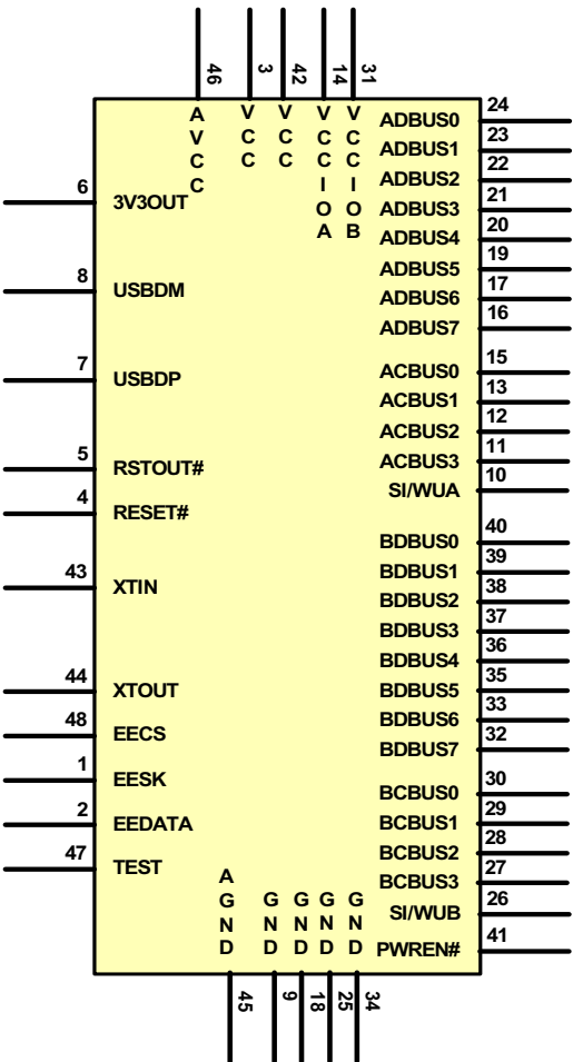
Figure 3 Pin-Out
