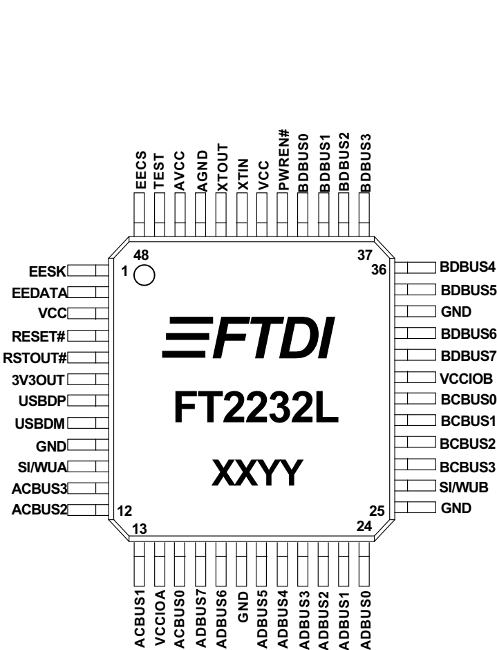
Figure 2 Pin-Out
