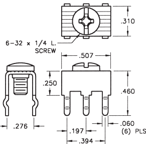
Mounting Detail
