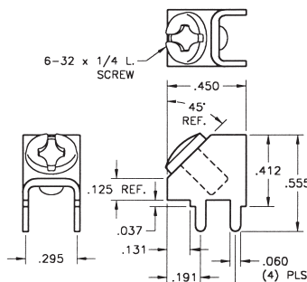
PC MOUNT
