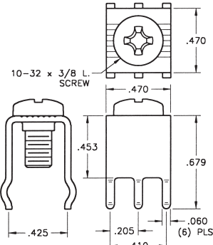
Mounting Detail
