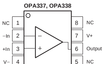
DIP-8 (1) , SO-8, MSOP-8 (1) NC = No Connection
