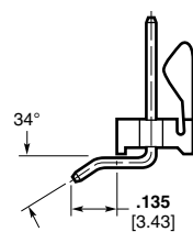
Retentive Leg
