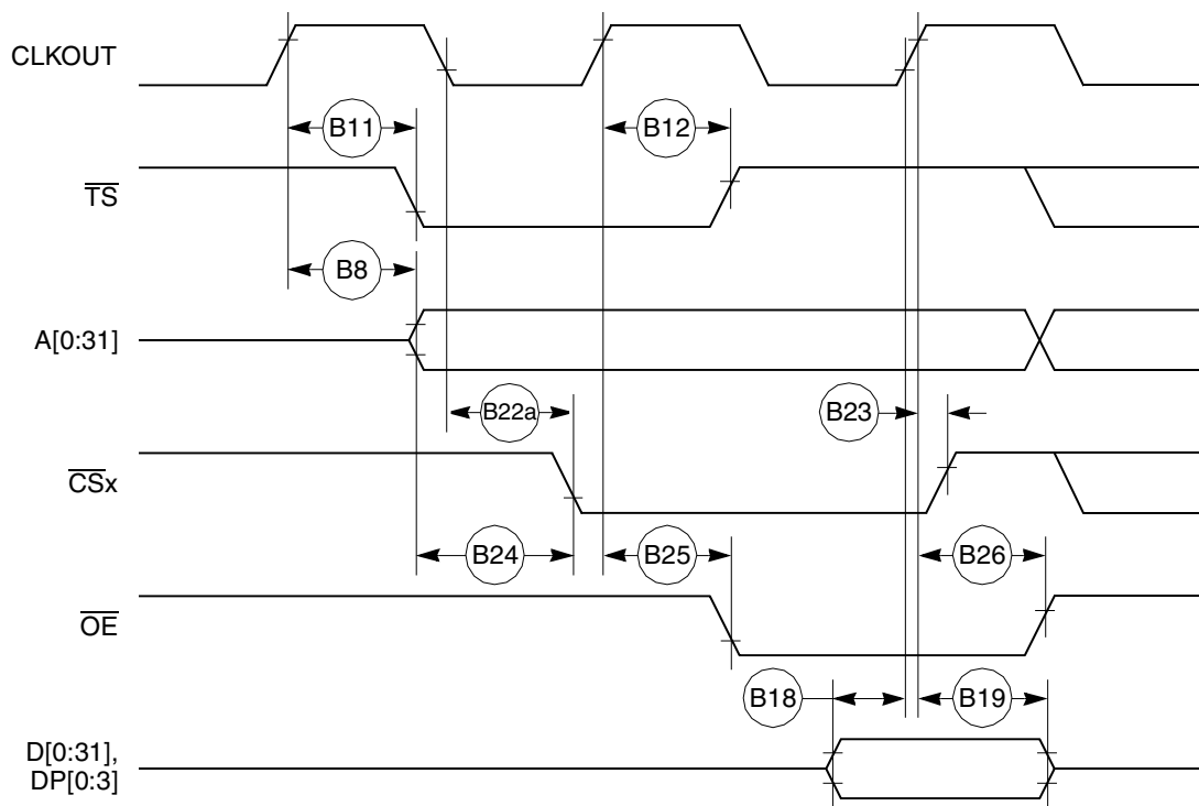
Figure 11. External Bus Read Timing (GPCM Controlled— TRLX = 0 , ACS = 10 )
