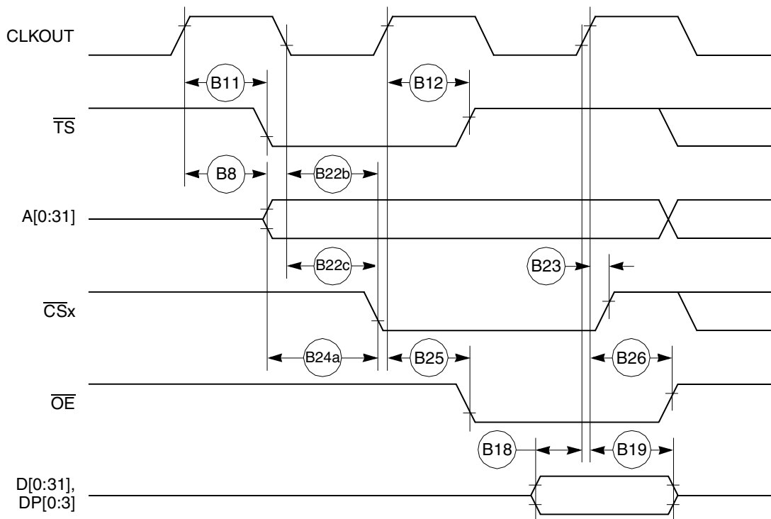
Figure 12. External Bus Read Timing (GPCM Controlled— TRLX = 0 , ACS = 11 )
