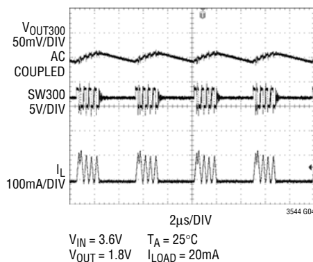
Burst Mode Operation 300mA Channel
