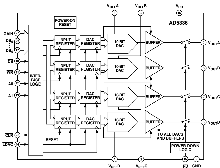
AD5336 PIN FUNCTION DESCRIPTIONS
