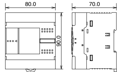
FC5A-C10R2, FC5A-C16R2 FC5A-C10R2C, FC5A-C16R2C
