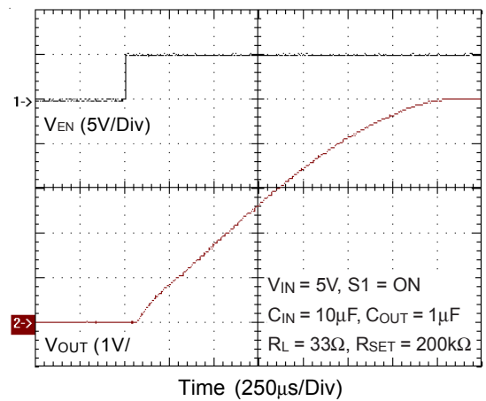
① Turn-On Response
