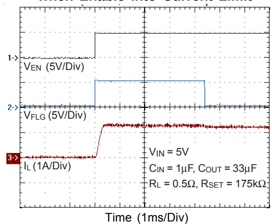
① FLAG Response when Enable into Current Limit
