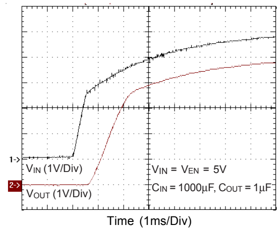
④ UVLO at Rising
