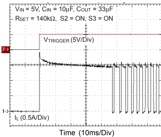
⑤ Short-Circuit with Thermal Shutdown
