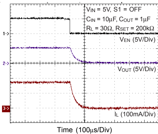
① Turn-Off Response
