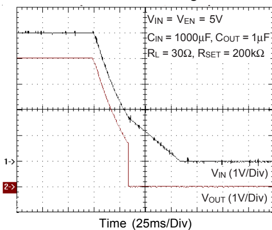
④ UVLO at Falling
