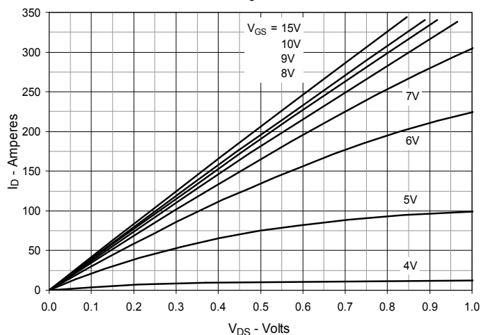
Fig. 3. Output Characteristics
