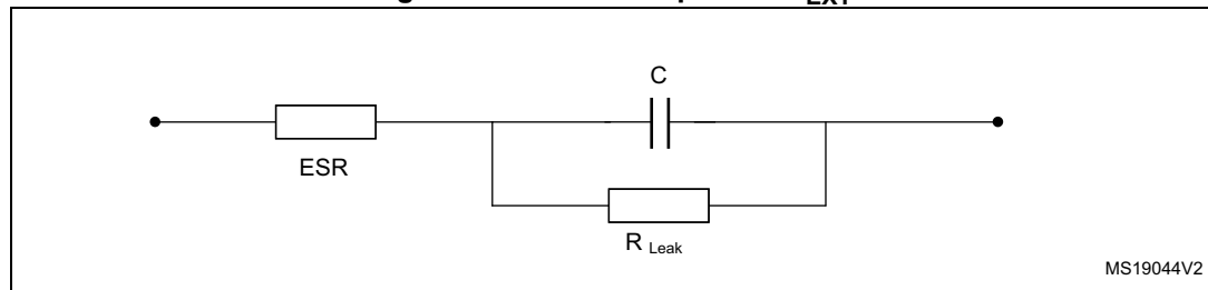
Figure 19. External capacitor C_{\text{EXT}}
