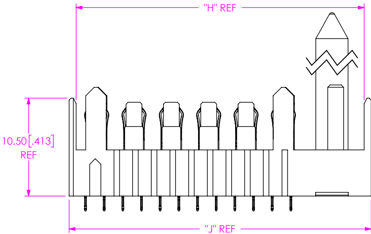
FIG 7 EBTM-6-12-2.0-X-VT-1-L-G-W SHOWN (EXCEPT AS SHOWN, SAME AS FIG 6) (NOT TOOLED)
