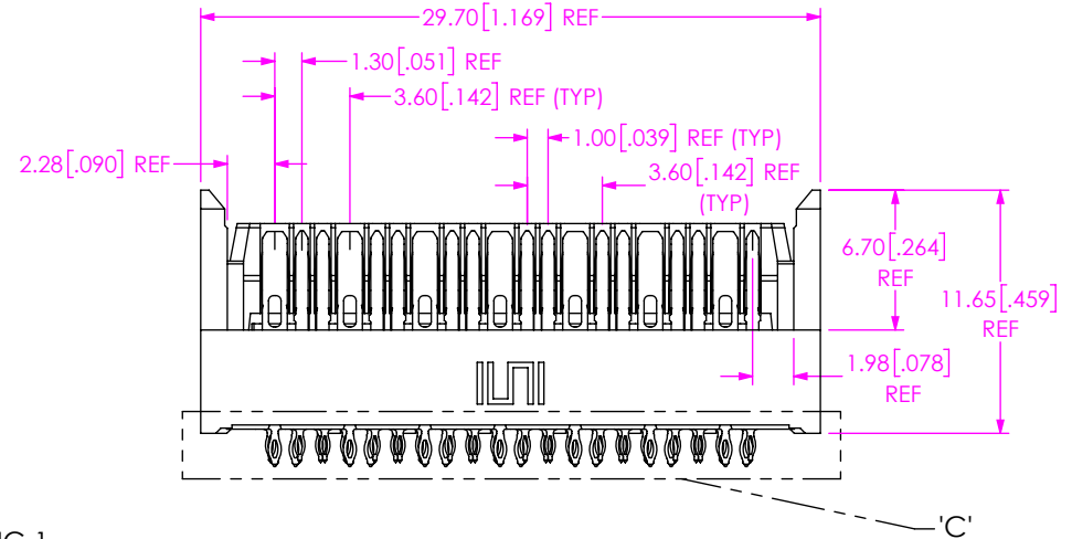
FIG 1 EBTM-6-12-2.0-X-VT-1 SHOWN
