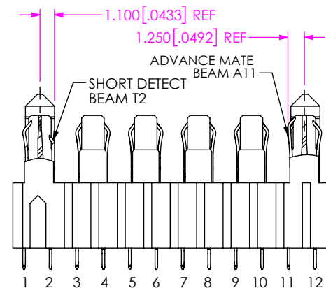
FIG 5 EBTM-6-12-2.0-X-VT-4 SHOWN (EXCEPT AS SHOWN, SAME AS FIGS 1, 3 & 4) (NOT TOOLED)
