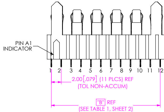
FIG 1 EBTM-6-12-2.0-X-VT-1 SHOWN
