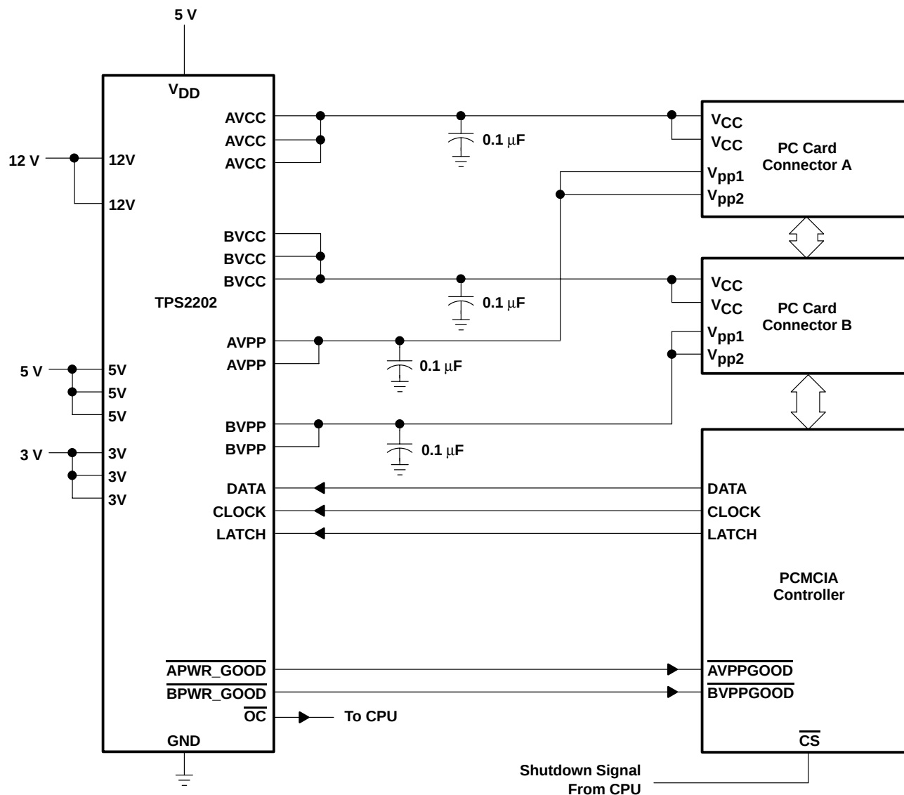
Figure 25. Detailed Interconnections and Capacitor Recommendations
