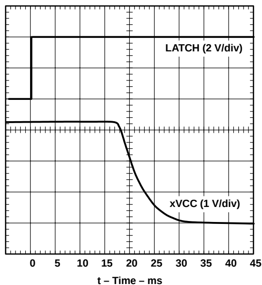
Figure 6. xVCC Propagation Delay and Fall Times With 100- \mu F Load, 3-V Switch
