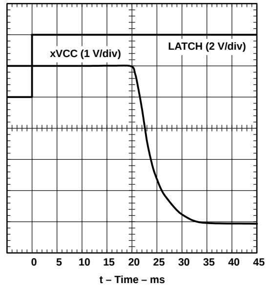
Figure 10. xVCC Propagation Delay and Fall Times With 100- \mu F Load, 5-V Switch
