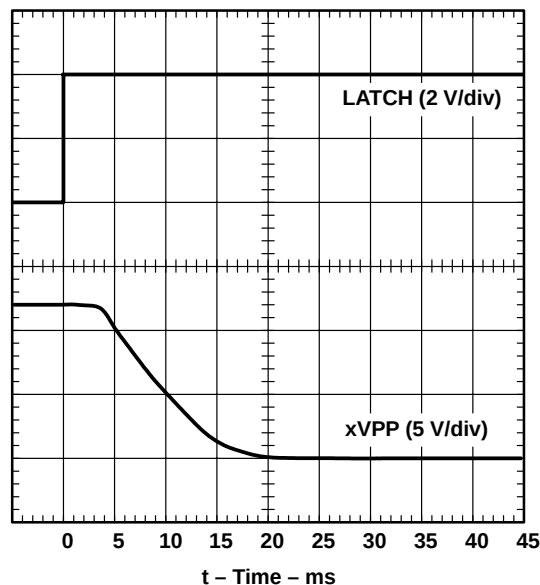
Figure 14. xVPP Propagation Delay and Fall Times With 100- \mu F Load, 12-V Switch
