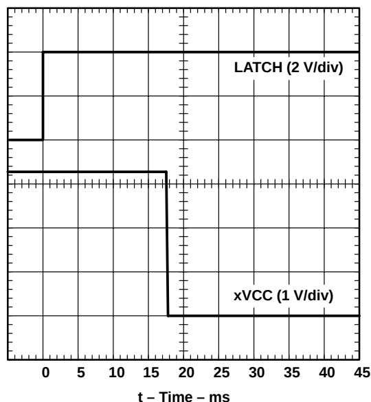
Figure 4. xVCC Propagation Delay and Fall Times With 1- \mu F Load, 3-V Switch
