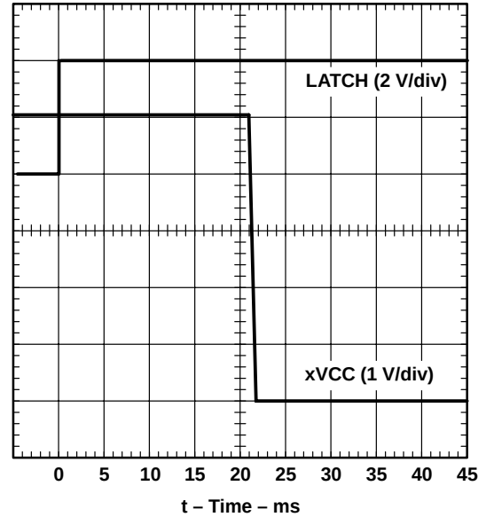
Figure 8. xVCC Propagation Delay and Fall Times With 1- \mu F Load, 5-V Switch
