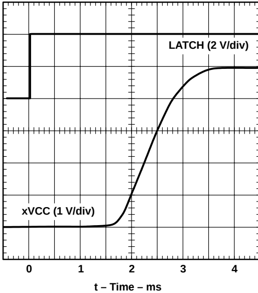
Figure 7. xVCC Propagation Delay and Rise Times With 1- \mu F Load, 5-V Switch
