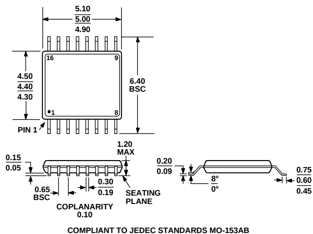
Figure 37.16. 16-Lead Thin Shrink Small Outline Package [TSSOP] (RU-16)
