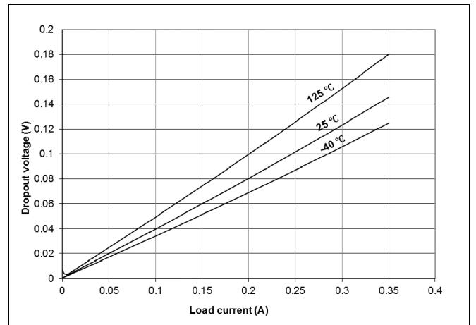
Figure 34. Dropout voltage - LDO4 - V_{OUT} = 1.8 V
