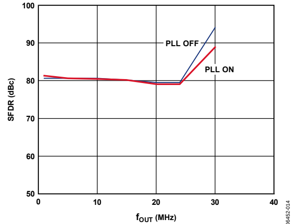
Figure 15. AD9779A In-Band SFDR vs. f_{OUT} , 4x Interpolation, f_{DATA} = 100 MSPS, PLL On/Off
