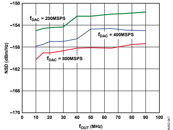
Figure 50. AD9776A Noise Spectral Density vs. f_{OUT} , Eight-Tone Input with 500 kHz Spacing, f_{DATA} = 200 \text{ MSPS}
