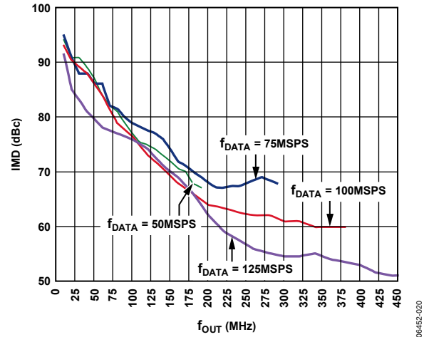
Figure 21. AD9779A Third-Order IMD vs. f_{OUT} , 8x Interpolation
