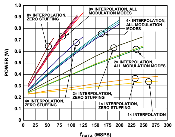
Figure 95. Total Power Dissipation, Dual DAC Mode
