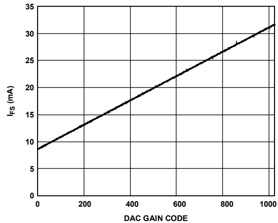
Figure 77. I_{\text{FS}} vs. DAC Gain Code
