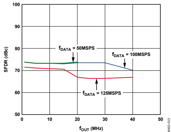
Figure 14. AD9779A Out-of-Band SFDR vs. f_{OUT} , 8x Interpolation
