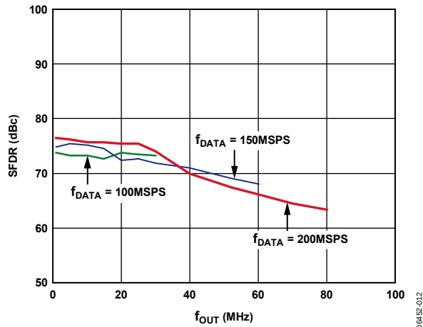
Figure 13. AD9779A Out-of-Band SFDR vs. f_{OUT} , 4x Interpolation
