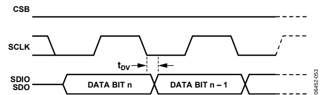
Figure 56. Timing Diagram for 3-Wire Interface Register Read
