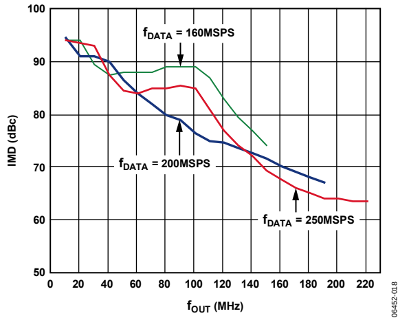
Figure 19. AD9779A Third-Order IMD vs. f_{OUT} , 2x Interpolation
