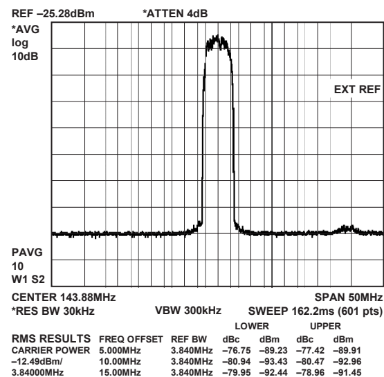
Figure 32. AD9779A W-CDMA Signal, 4× Interpolation, f_{DATA} = 122.88 MSPS, f_{DAC}/4 Modulation
