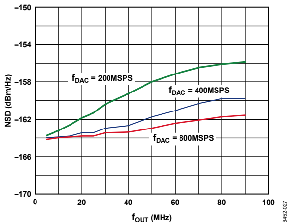
Figure 30. AD9779A Noise Spectral Density vs. f_{OUT} , f_{DAC} Over Output Frequency with a Single-Tone Input at -6 dBFS
