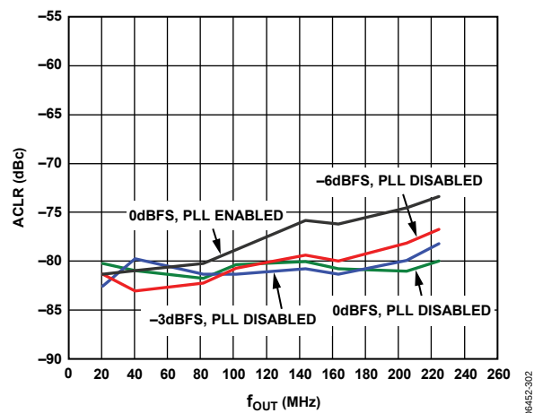
Figure 34. AD9779A ACLR for Third Adjacent Band W-CDMA, 4× Interpolation, f_{DATA} = 122.88 MSPS, On-Chip Modulation Translates Baseband Signal to IF
