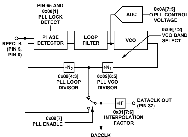
Figure 72. Clock Multiplier Circuit
