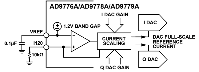
Figure 76. Reference Circuitry
