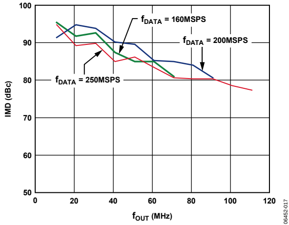
Figure 18. AD9779A Third-Order IMD vs. f_{OUT} , 1x Interpolation
