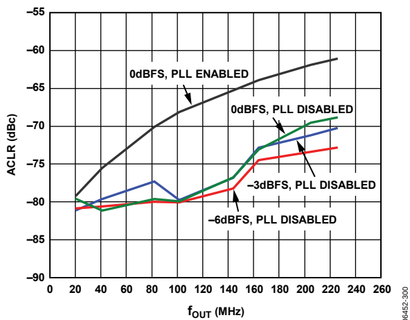
Figure 31. AD9779A ACLR for First Adjacent Band W-CDMA, 4× Interpolation, f_{DATA} = 122.88 MSPS, On-Chip Modulation Translates Baseband Signal to IF
