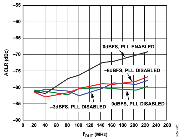
Figure 33. AD9779A ACLR for Second Adjacent Band W-CDMA, 4× Interpolation, f_{DATA} = 122.88 MSPS, On-Chip Modulation Translates Baseband Signal to IF
