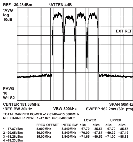
Figure 35. AD9779A Multicarrier W-CDMA Signal, 4× Interpolation, f_{DAC} = 122.88 MSPS, f_{DAC}/4 Modulation
