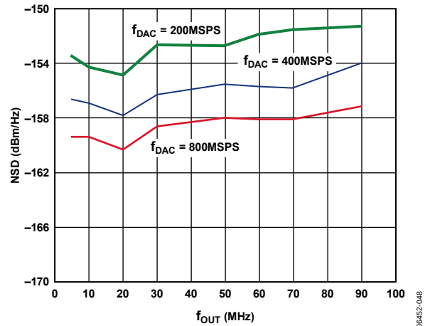
Figure 51. AD9776A Noise Spectral Density vs. f_{OUT} , Single-Tone Input at -6 \text{ dBFS} , f_{DATA} = 200 \text{ MSPS}
