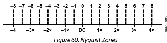
Figure 60. Nyquist Zones
