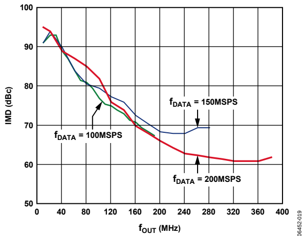
Figure 20. AD9779A Third-Order IMD vs. f_{OUT} , 4x Interpolation
